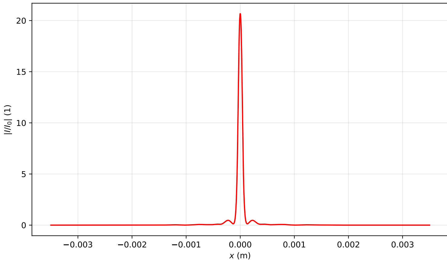
Intensity profile I(x, y = 0, z = 1.672)/I_0 , P_{in}=5.0P_{cr} , artificial time
